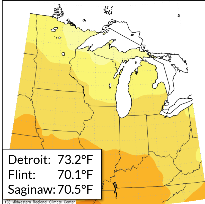
Average Temperature (°F) June 1, 2022 to August 31, 2022
