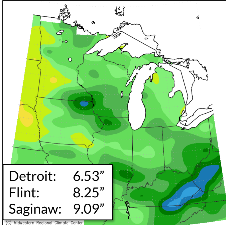
Accumulated Precipitation (in) June 1, 2022 to August 31, 2022
