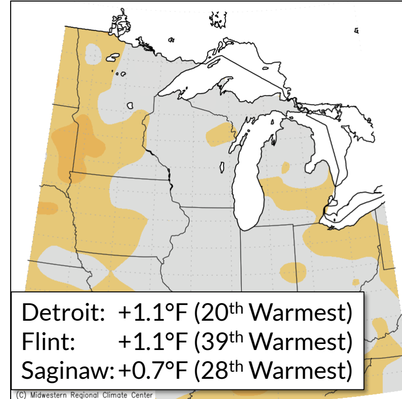
Average Temperature (°F): Departure from Mean June 1, 2022 to August 31, 2022
