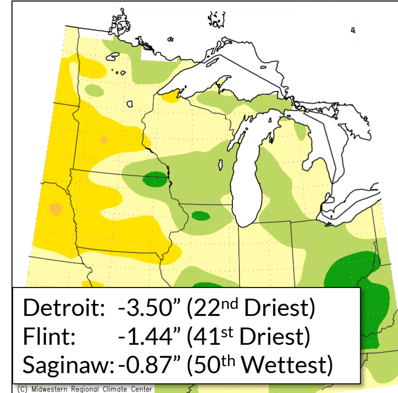
Accumulated Precipitation: Percent of Mean June 1, 2022 to August 31, 2022
