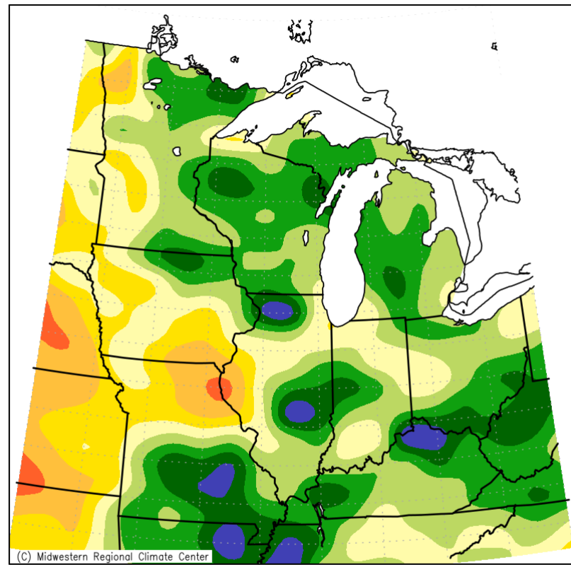
Accumulated Precipitation: Percent of Mean August 1, 2022 to August 31, 2022
