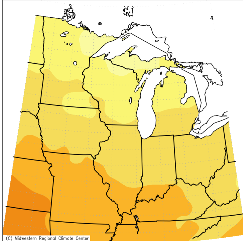
Average Temperature (°F) August 1, 2022 to August 31, 2022
