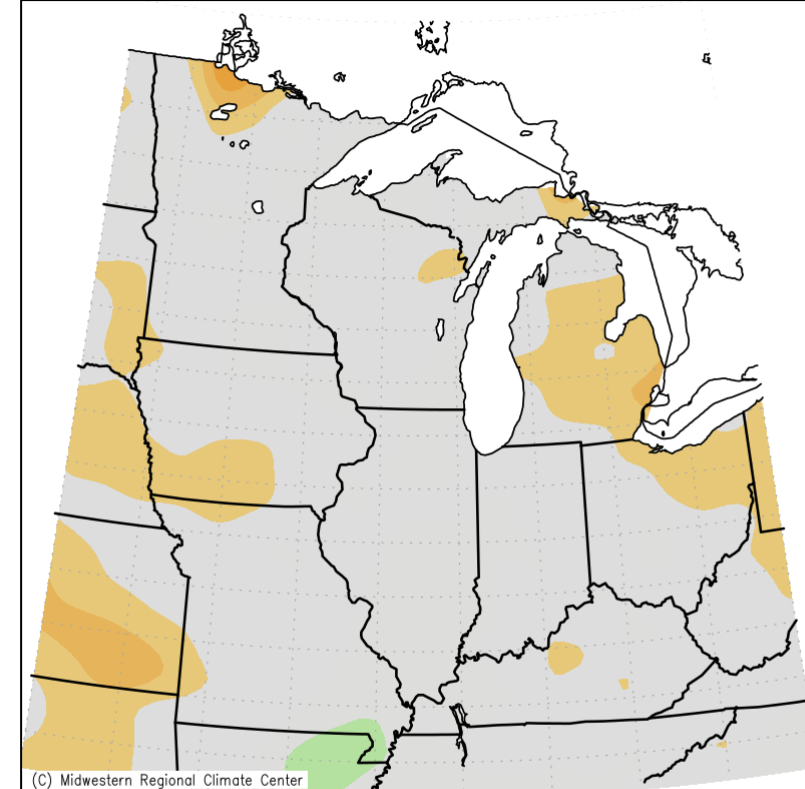
Average Temperature (°F): Departure from Mean August 1, 2022 to August 31, 2022
