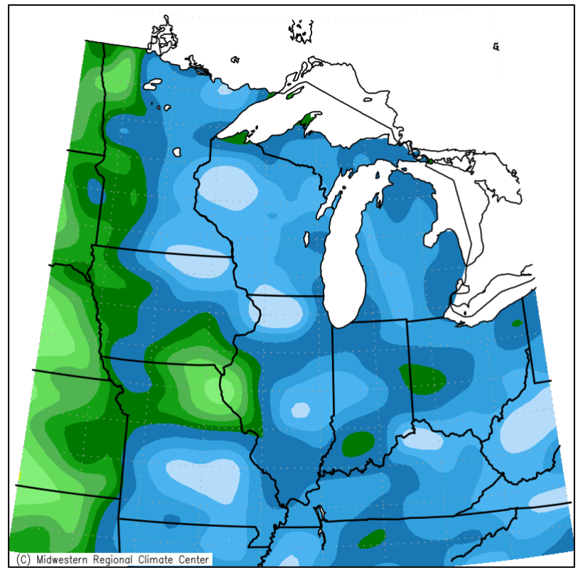
Accumulated Precipitation (in) August 1, 2022 to August 31, 2022
