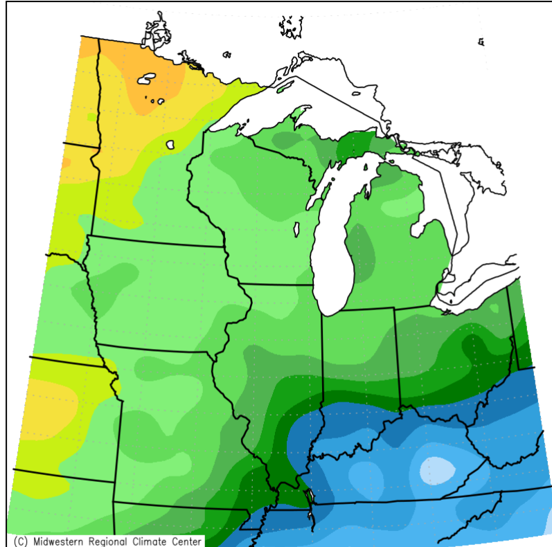
Accumulated Precipitation (in) February 1, 2021 to February 28, 2021
