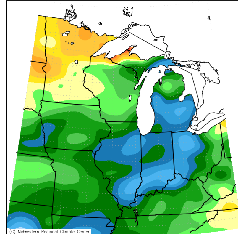
Accumulated Snowfall (in): Departure from Mean February 1, 2021 to February 28, 2021
