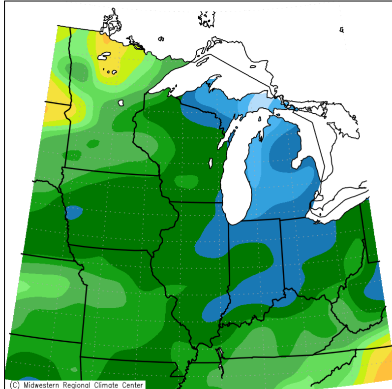
Accumulated Snowfall (in) February 1, 2021 to February 28, 2021
