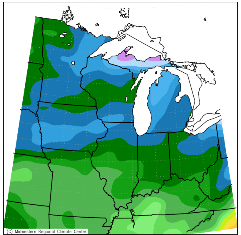
Accumulated Snowfall (in) October 1, 2020 to February 28, 2021
