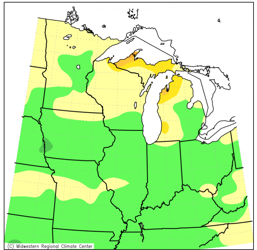
Accumulated Snowfall (in): Departure from Mean October 1, 2020 to February 28, 2021
